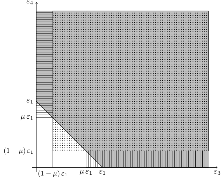
Figure 3.1: ( \varepsilon = 3 , \mu = 3/4 ) The domain of integration of the integral J_1 , in grey, is covered by the union of the domain with points, the domain with vertical lines and that with horizontal lines. In the part of the grey domain covered by points the function W is bounded by one. In the part of vertical and horizontal lines the grey domain covered by vertical lines it is less than or equal to \sqrt{\varepsilon_4}/\sqrt{\varepsilon_3} .
