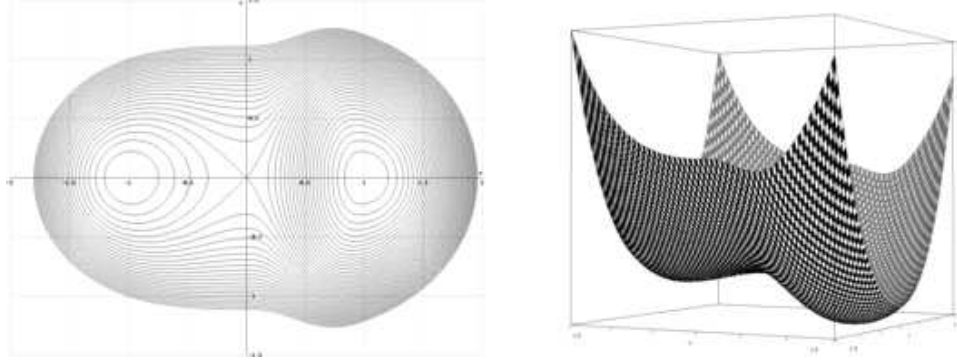
Fig. 1: Simulation of the standard 2-well W deformed (exmpl. 35), having minima at different levels
